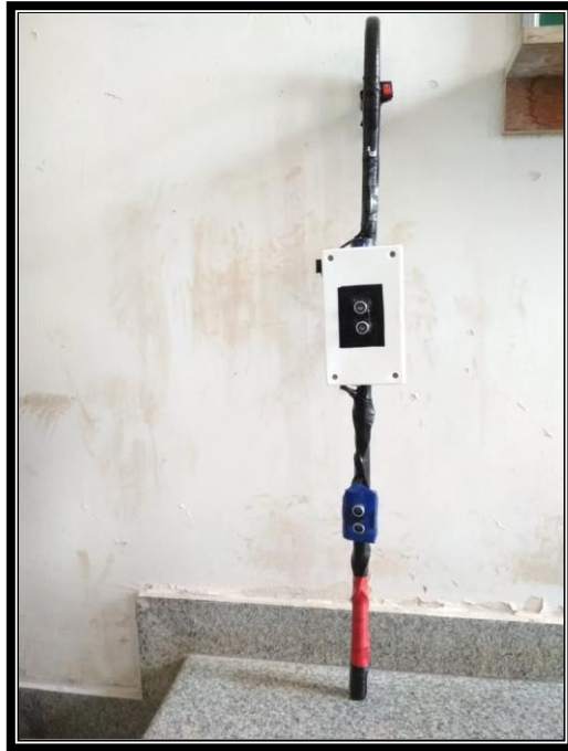
Blind man Smart Stick
